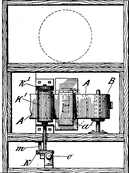
SECTION. ZZ OF FIG. 2.
